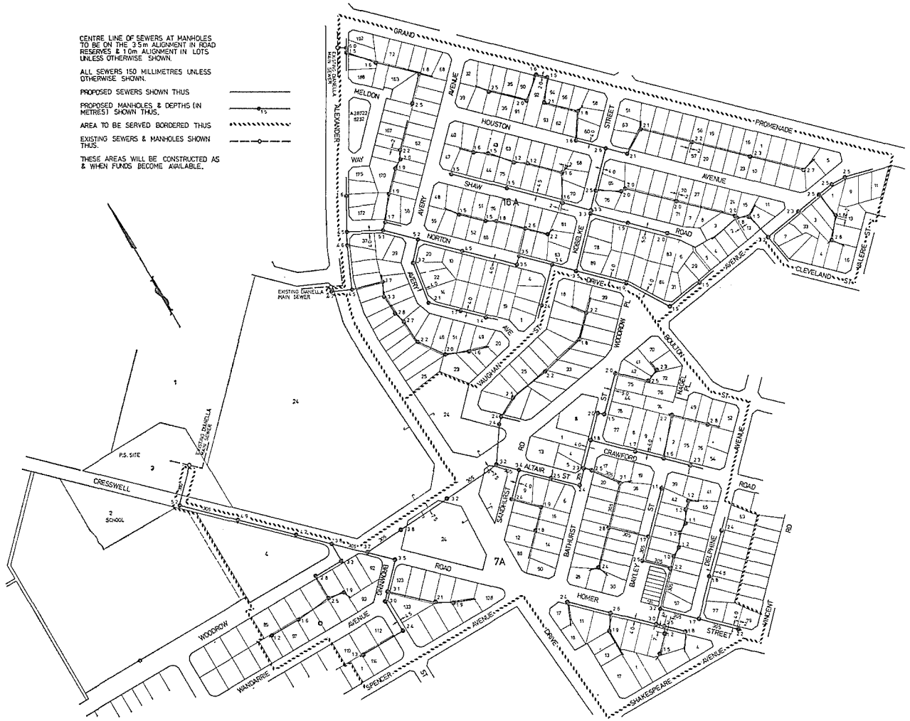
METROPOLITAN SEWERAGE RETICULATION AREAS 7A & 16A MORLEY M.W.B. 13067
