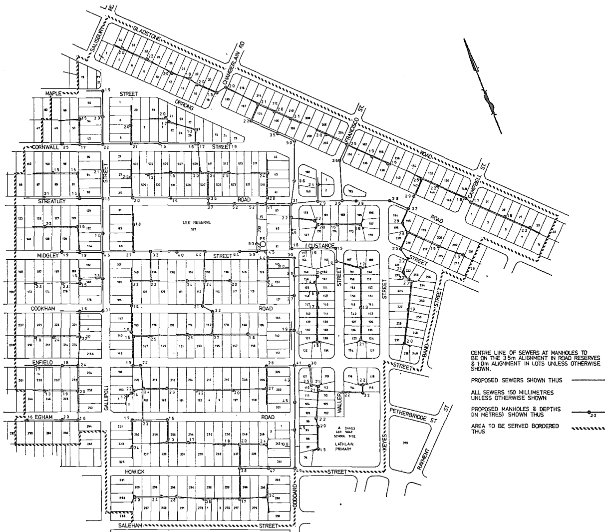
METROPOLITAN SEWERAGE RETICULATION AREA 5A RIVERVALE M.W.B. 13320
