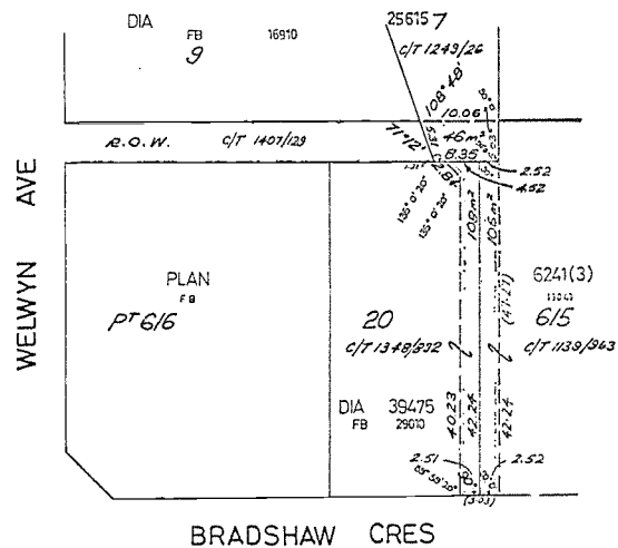
Compiled From Diagrams 25615 and 39475 and Plan 6241(3)
