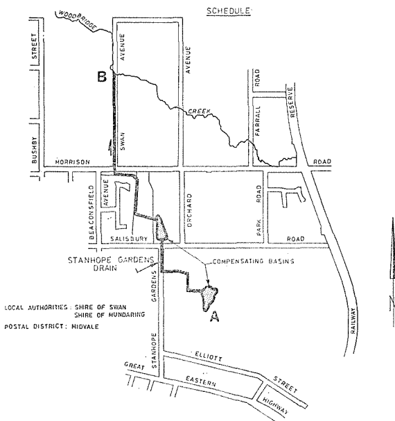
METROPOLITAN WATER BOARD PERTH W.A. CONSTITUTION OF STANHOPE GARDENS MAIN DRAIN - MIDVALE SCALE 10 000 SHEET PERTH 5.7
