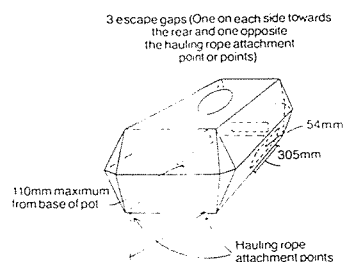
DIAGRAM 8 - PLASTIC POTS (Clause 5(b))
