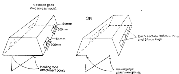
DIAGRAM 5 - BATTEN POTS (Clause 4(c)(i)) (Steel Flat-Bar)
