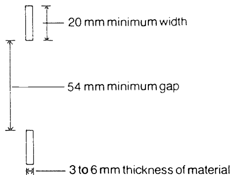
DIAGRAM 5 - BATTEN POTS (Clause 4(c)(i)) (Steel Flat-Bar)
