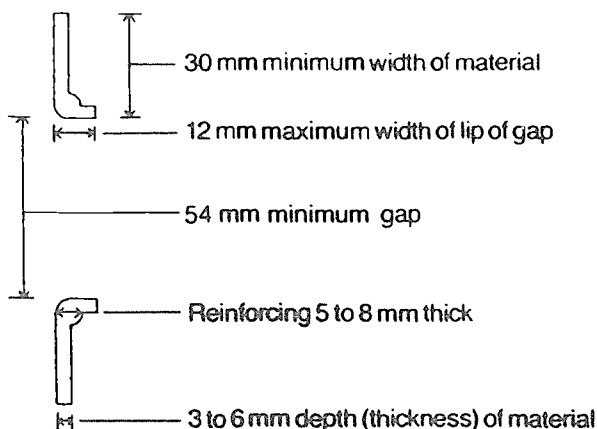
DIAGRAM 7 - BATTEN POTS (Clause 4(c)(iii)) (Fibreglass)
