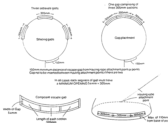
DIAGRAM 2 - OTHER POTS (Clause 3(d))
