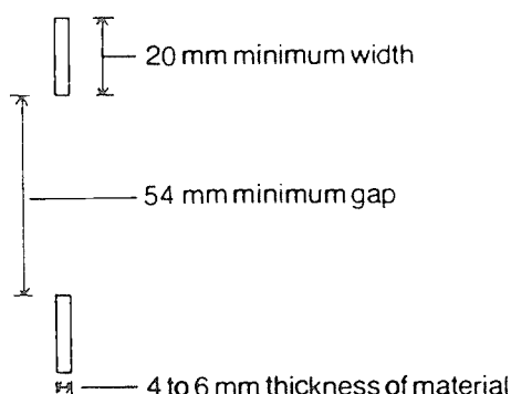
DIAGRAM 6 - BATTEN POTS (Clause 4(c)(ii)) (Aluminium)
