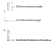
DIAGRAM 1 - OTHER POTS (Clause 3(b)) (Steel Flat-Bar)
