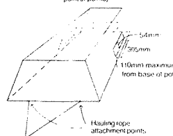
DIAGRAM 3 - BATTEN POTS (Clause 4(b)(i))
