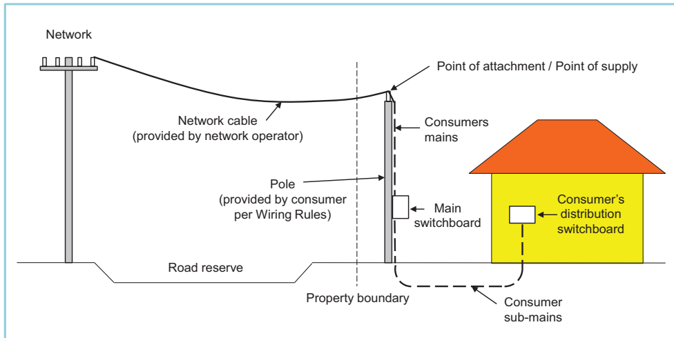
Figure 3.3 Overhead supply to consumer's pole/main switchboard
