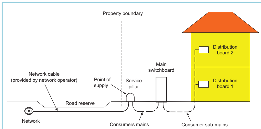
Figure 3.7 Typical underground service to multi-lot built strata
