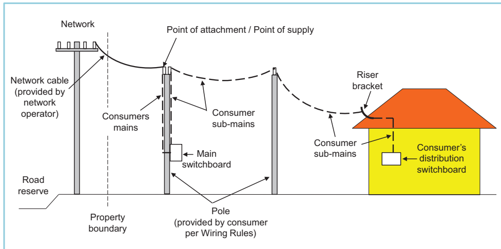
Figure 3.4 Overhead supply to rural consumer 2
