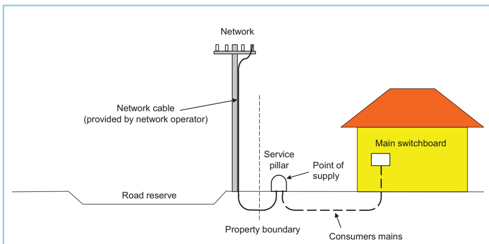
Figure 3.5 Overhead street mains and underground consumers mains
