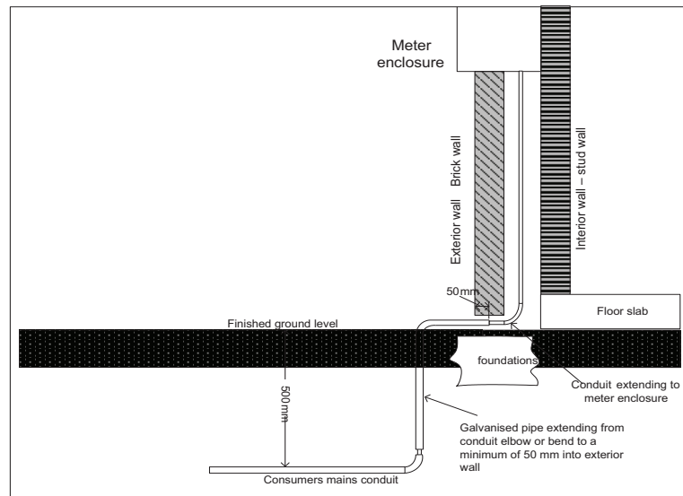
Figure 9.4(d) Conduit entry through wall - brick veneer
