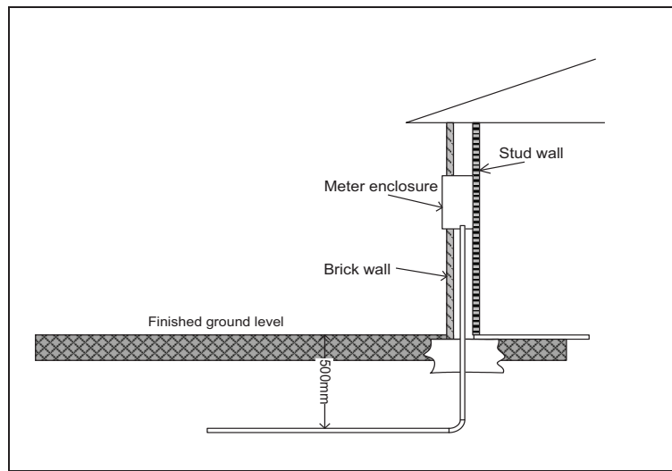
Figure 9.4(b) Conduit entry through slab - brick veneer
