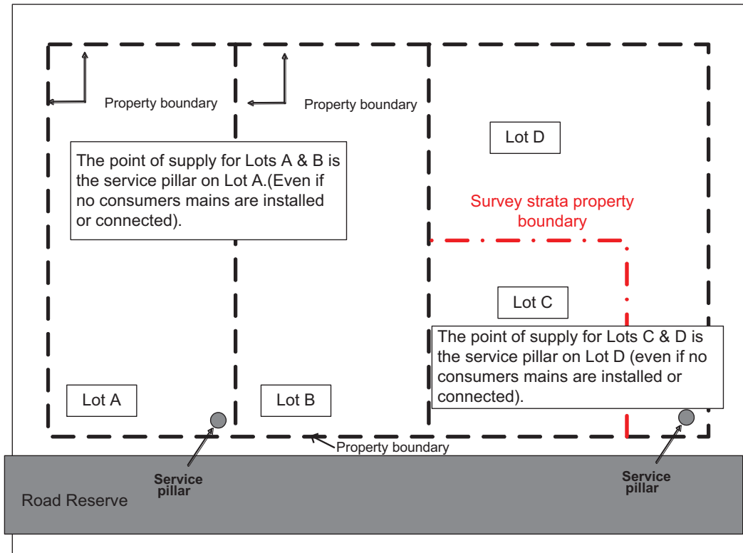
Figure 3.8(a) Example of points of supply
