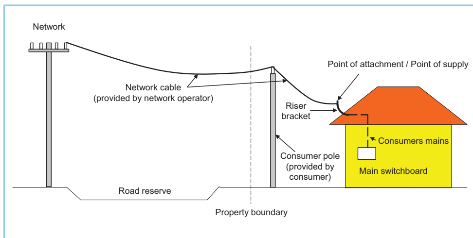
Figure 3.2 Overhead service with consumer pole
