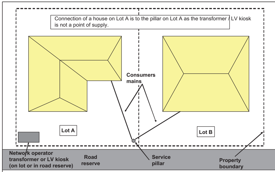
Figure 3.8(c) Example of points of supply
