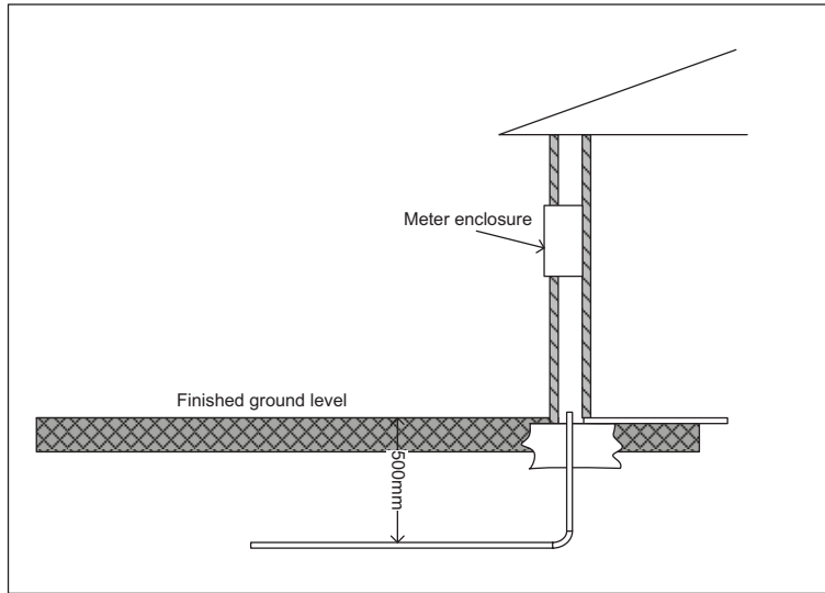
Figure 9.4(a) Conduit entry through slab – double brick
