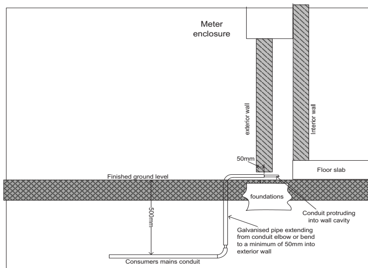
Figure 9.4(c) Conduit entry through wall – double brick
