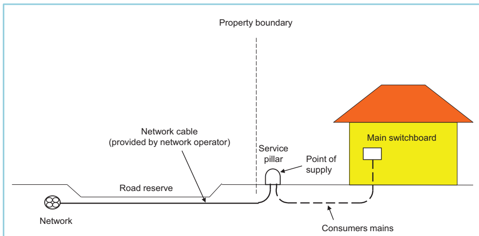
Figure 3.6 Underground network and underground consumers mains
