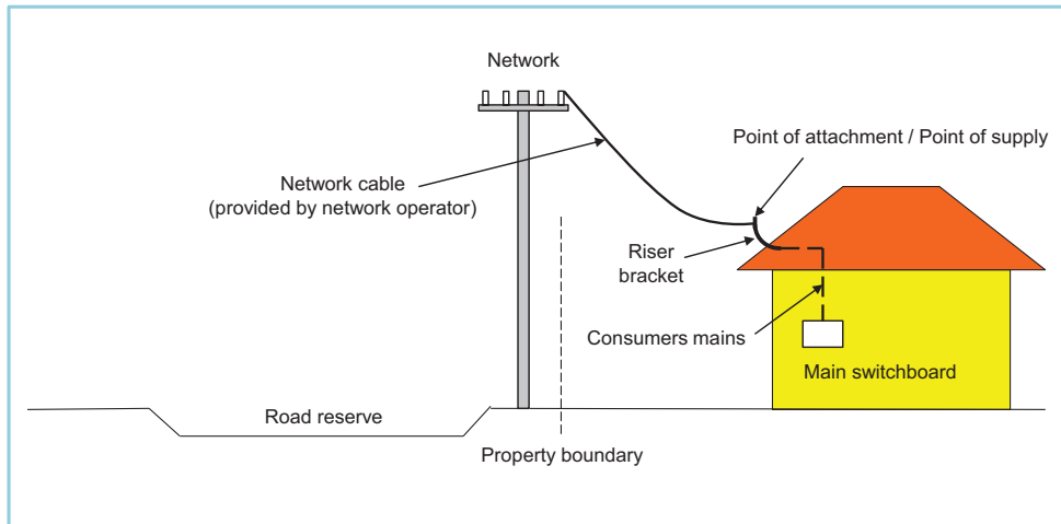
Figure 3.1 Overhead service
