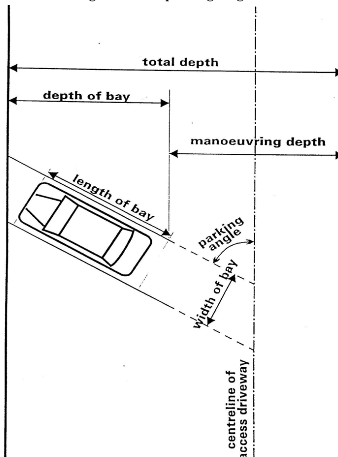
Figure 1—Car parking diagram
