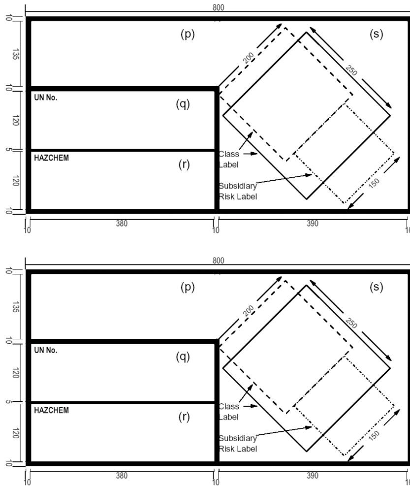
Figure 2 — Template for a placard for dangerous goods (other than C1 combustible liquids) in bulk
