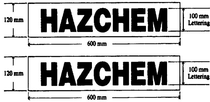
Figure 1 — Form and dimensions of an outer warning placard
