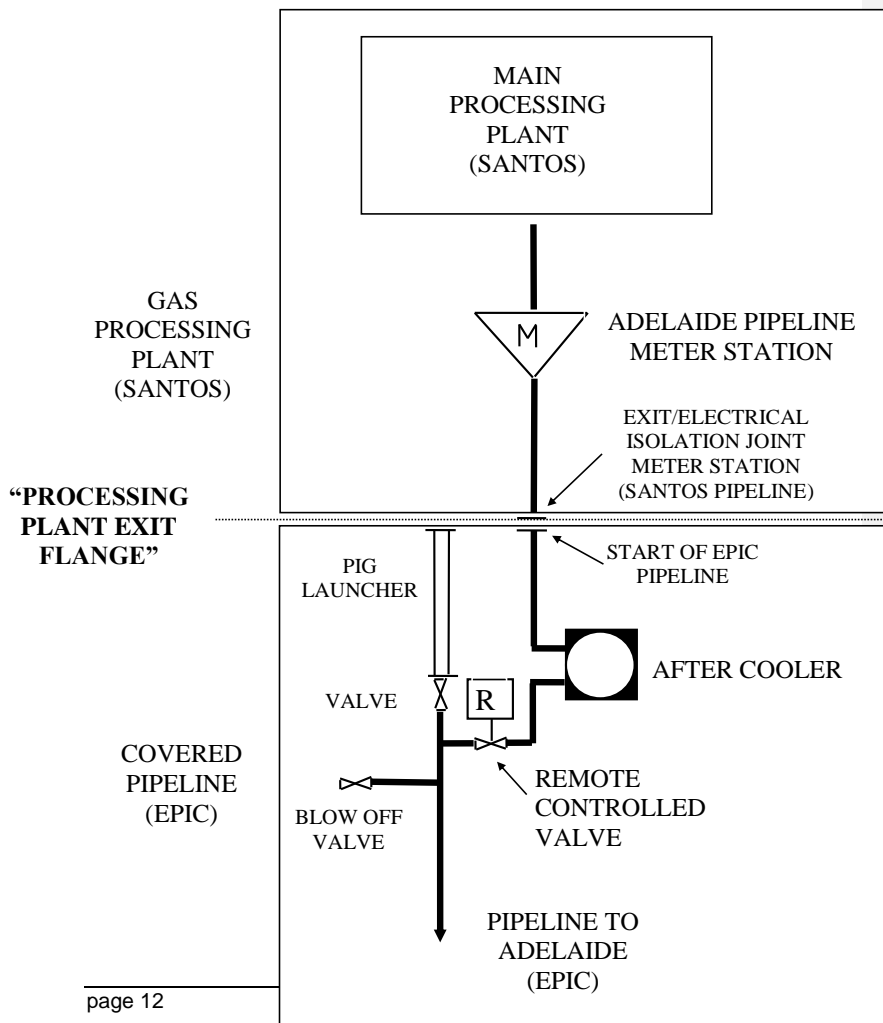
DIAGRAM 1 MOOMBA PLANT PRESCRIBED PLANT AND EXIT FLANGE - MOOMBA TO ADELAIDE PIPELINE
