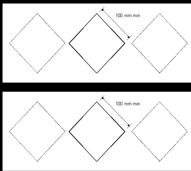
Figure 3 — Form and dimensions of a placard for storage of packaged dangerous goods
