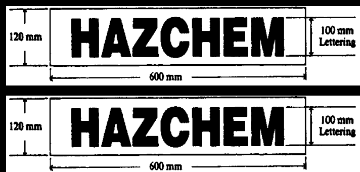
Figure 2 — Template for a placard for dangerous goods (other than C1 combustible liquids) in bulk
