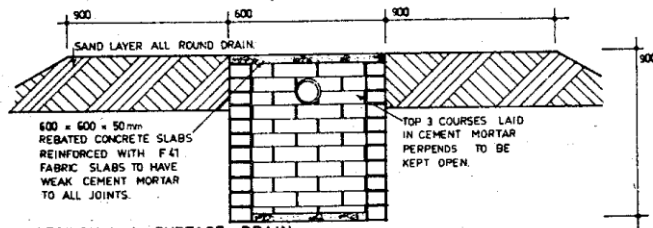
SECTION A-A SURFACE DRAIN.
