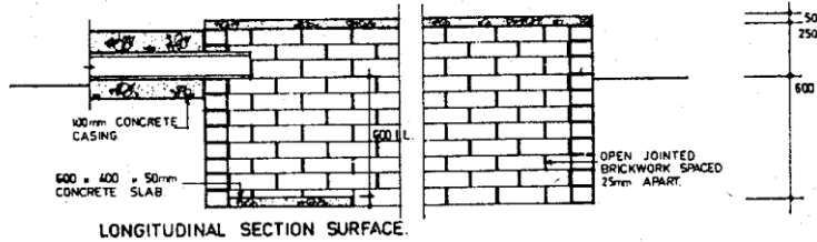
LONGITUDINAL SECTION SURFACE.
