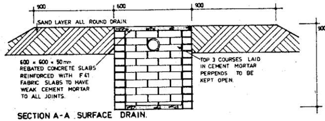
SECTION A-A SURFACE DRAIN.
