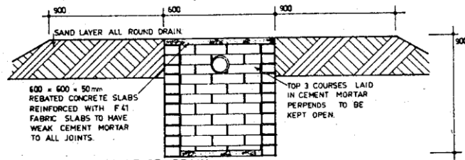
SECTION A-A SURFACE DRAIN.
