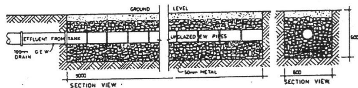
STANDARD FRENCH DRAIN
