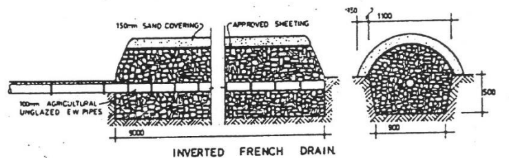
INVERTED FRENCH DRAIN
