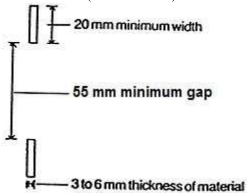
Diagram 4 — Batten Pots
