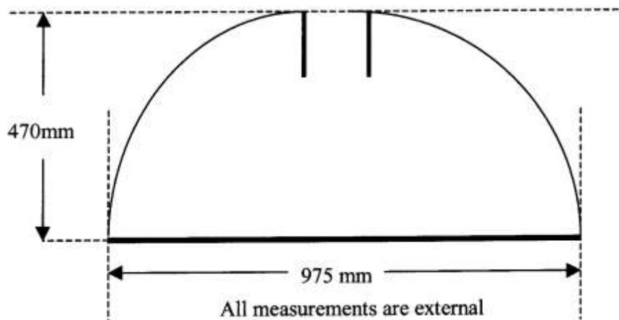
Diagram 10 — Beehive Pots
