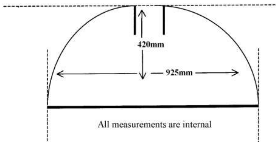
Diagram 11 — Beehive Pots
