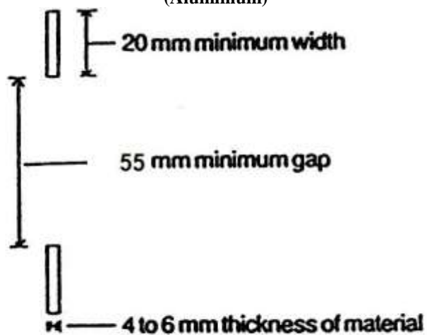
Diagram 5 — Batten Pots
