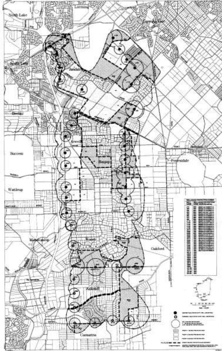
Plan 4 — Jandakot Underground Water Pollution Control Area
