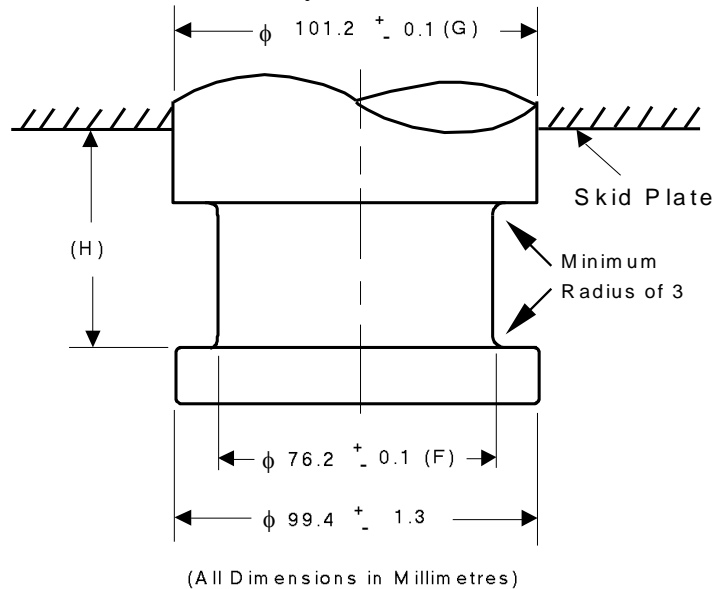
Dimensions of a 75 mm kingpin
