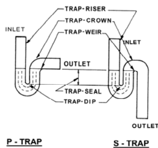
FIGURE 1.2 TRAPS
